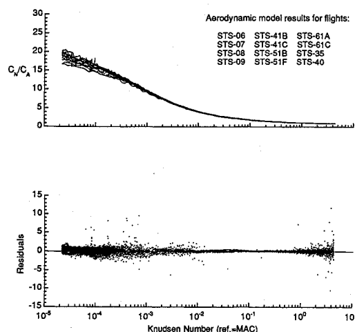
Fig. 10 C_N/C_A model results and HiRAP flight measurement comparisons.
