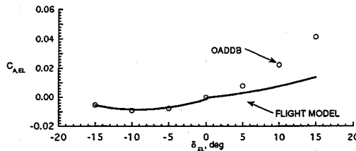
b) Axial axis coefficient increment
