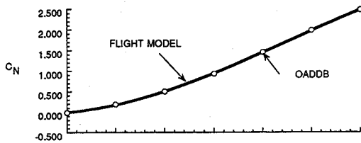
a) Normal axis coefficient
