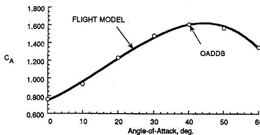
b) Axial axis coefficient
