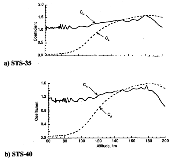
Fig. 16 Flight aerodynamic model force coefficients.
