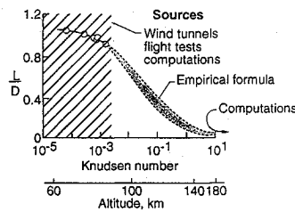
Fig. 1 Orbiter rarefied-flow aerodynamics status during early 1980s.
