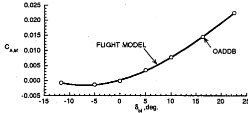
b) Axial axis coefficient increment
