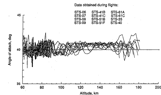
a) Orbiter angle of attack during re-entry
