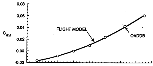
a) Normal axis coefficient increment
