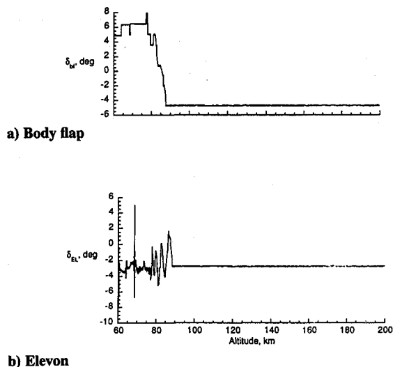
Fig. 15 Orbiter control surface settings for STS-40.
